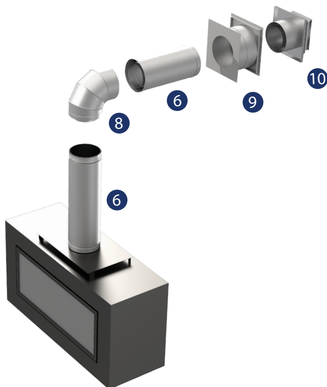
Installation horizontale
